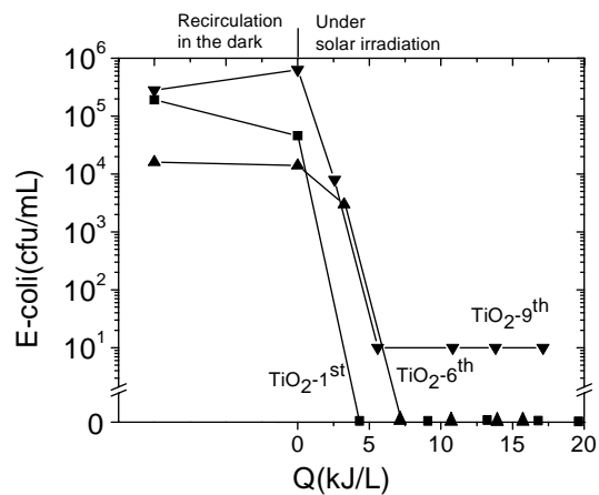
Figure 3: E-coli concentration as a function of integrated UV-A received energy by the photocatalytic reactor CPC type (Fig. 1).
